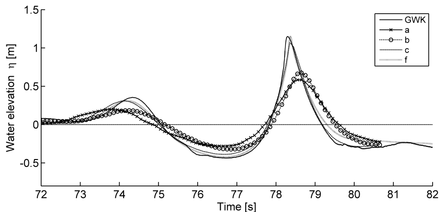
Figure 5.4: Wave gauge signal from large wave flume experiments (GWK) at the tripod position in comparison to time series of CFD simulations with meshes a, b, c, f in the quasi 2D model as listed in table 5.1.
