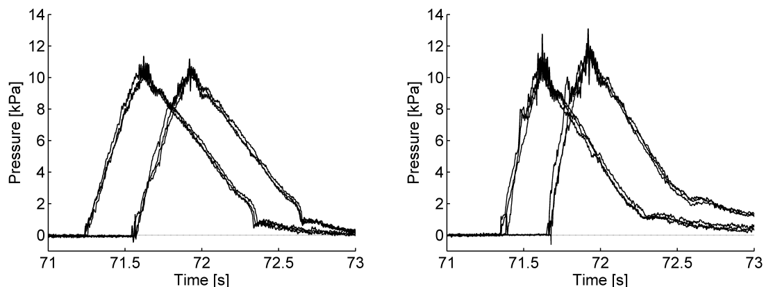
Figure 4.1: Similarity of hydrodynamic pressures at height z = 0.14 * \eta_{max} (left) and z = 0.33 * \eta_{max} (right) for different test waves.
