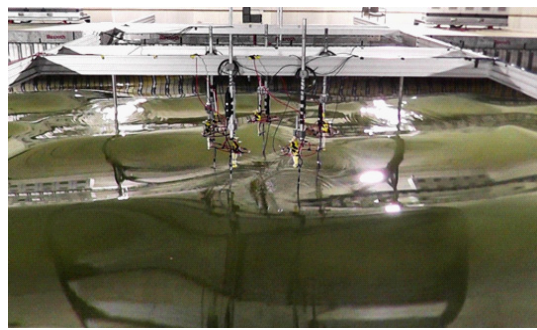
Abb. 2: Bichromatic-Bidirectional waves tested at the 3D wave basin in Marienwerder
